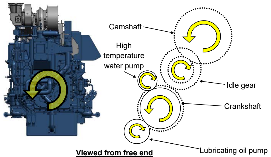
Figure 1.2 Direction of engine rotation
