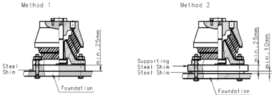
Figure 2.5 Recommendations for seating design
