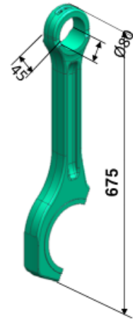
Connecting rod shaft Approx. 14.1 kg
