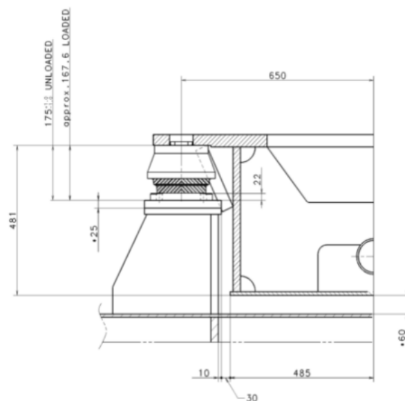
Figure 2.4 Resilient mounting
