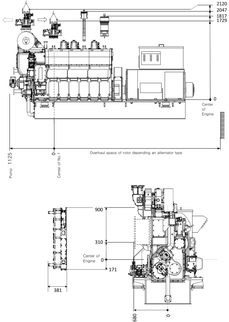
Figure 2.7 Overhaul dimension
