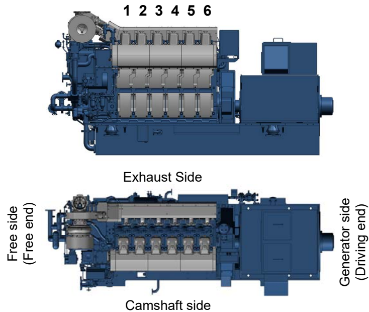
Figure 1.1 Cylinder numbering
